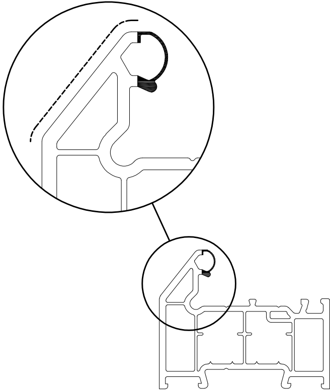
Chamfered Profile
