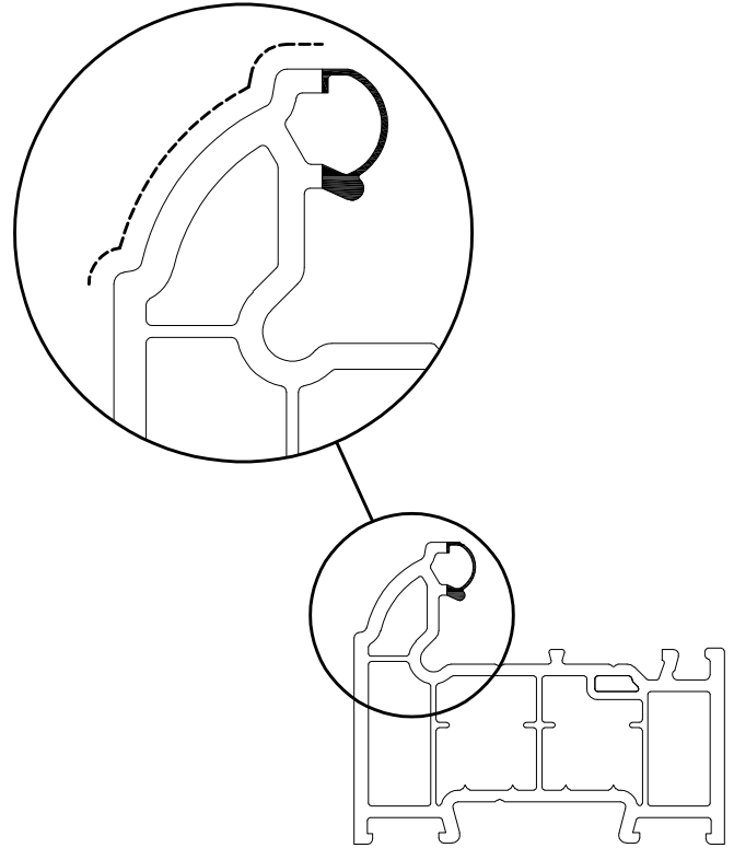
Sculptured Profile
